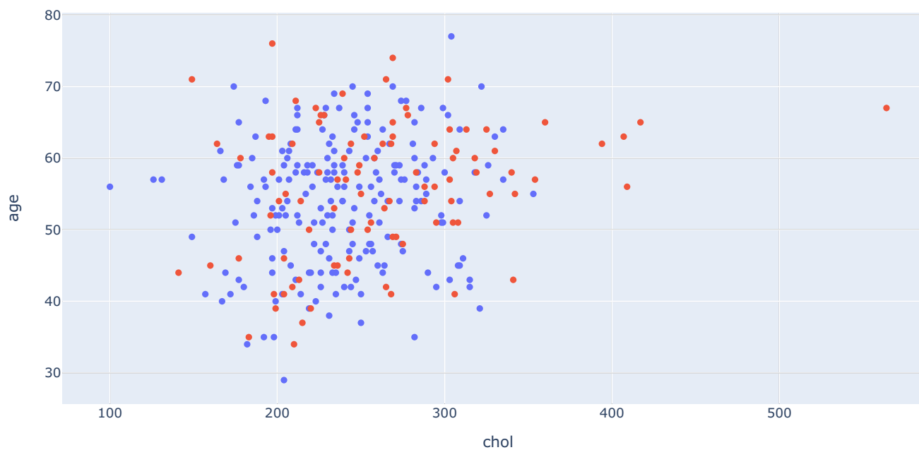
Scatter Plot of Cholesterol vs. Age (colored by Sex)
