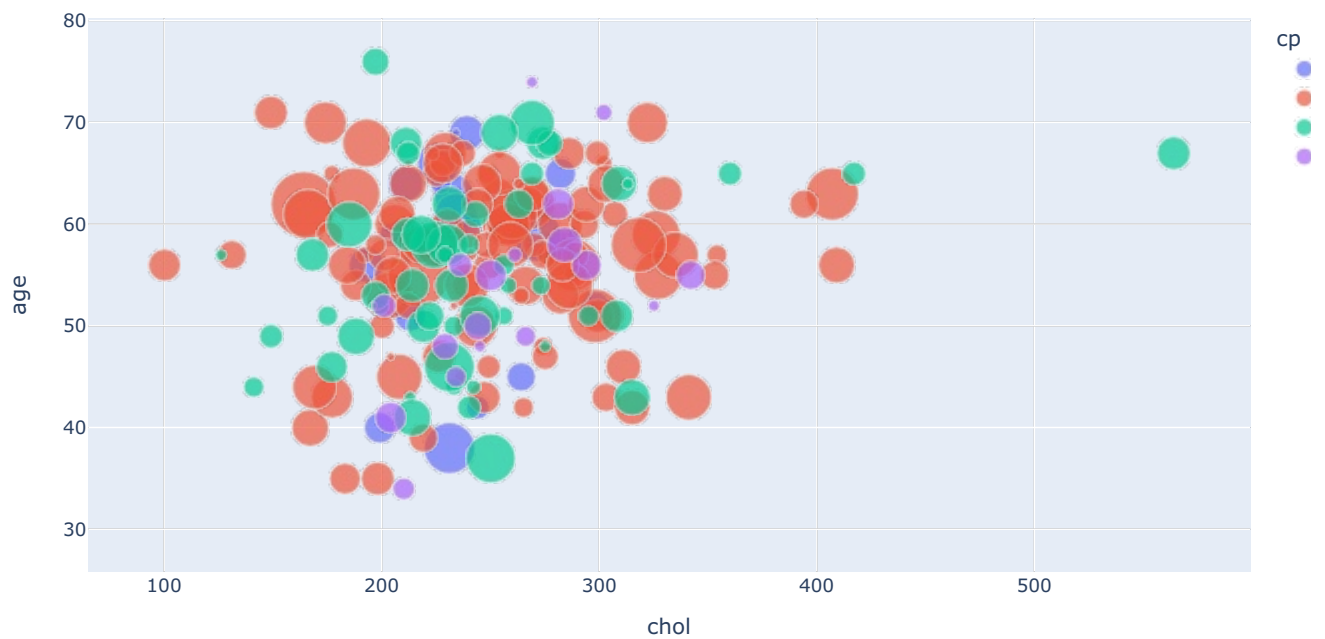
Scatter Plot of Cholesterol vs. Age (colored by cp)
