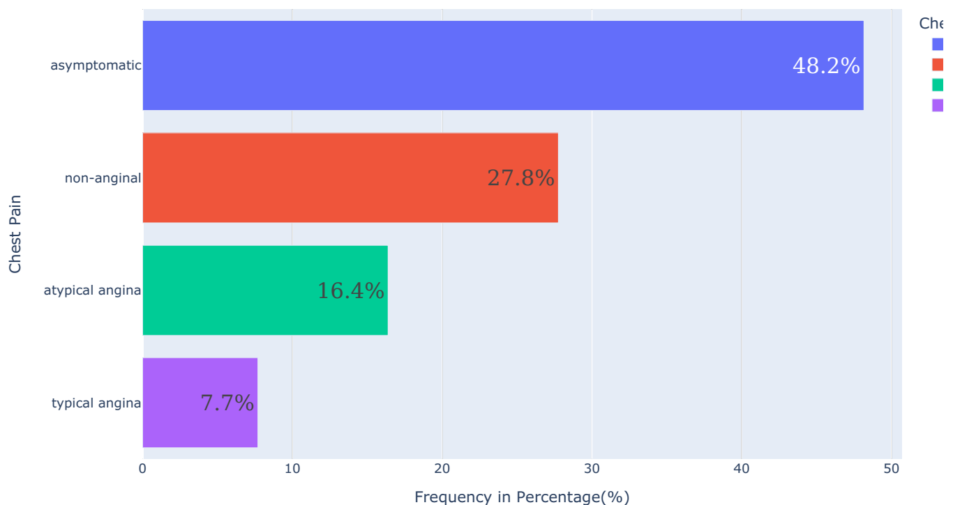
Frequency of Chest Pain
