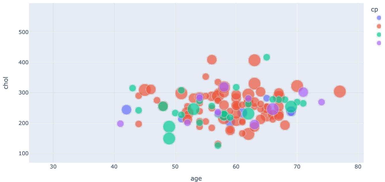
Cholesterol Vs Age
