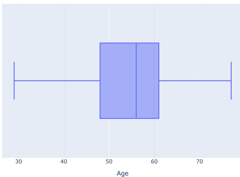
5-Number-Summary(Box Plot) of Age
